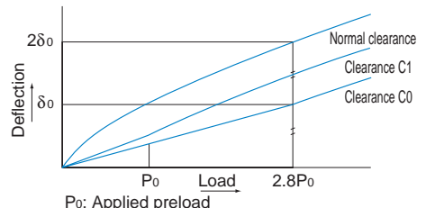
Fig.5 Rigidity Data
