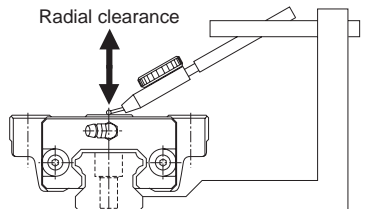
Fig.3 Radial clearance of the LM Guide
